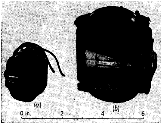
FIG. 13-3.—Core-and-coil assemblies of oil-filled pulse transformers (a) 120 kw (232BW2), 0.5 to 2.0 \mu sec. (b) 600 kw (410AW2) 0.5 to 2.0 \mu sec.
